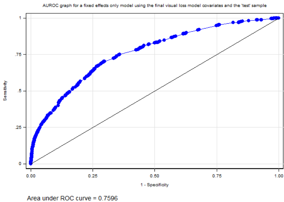
Figure 8: AUROC graph from a fixed effects only model of the final VA loss model covariates using the 'test' sample
