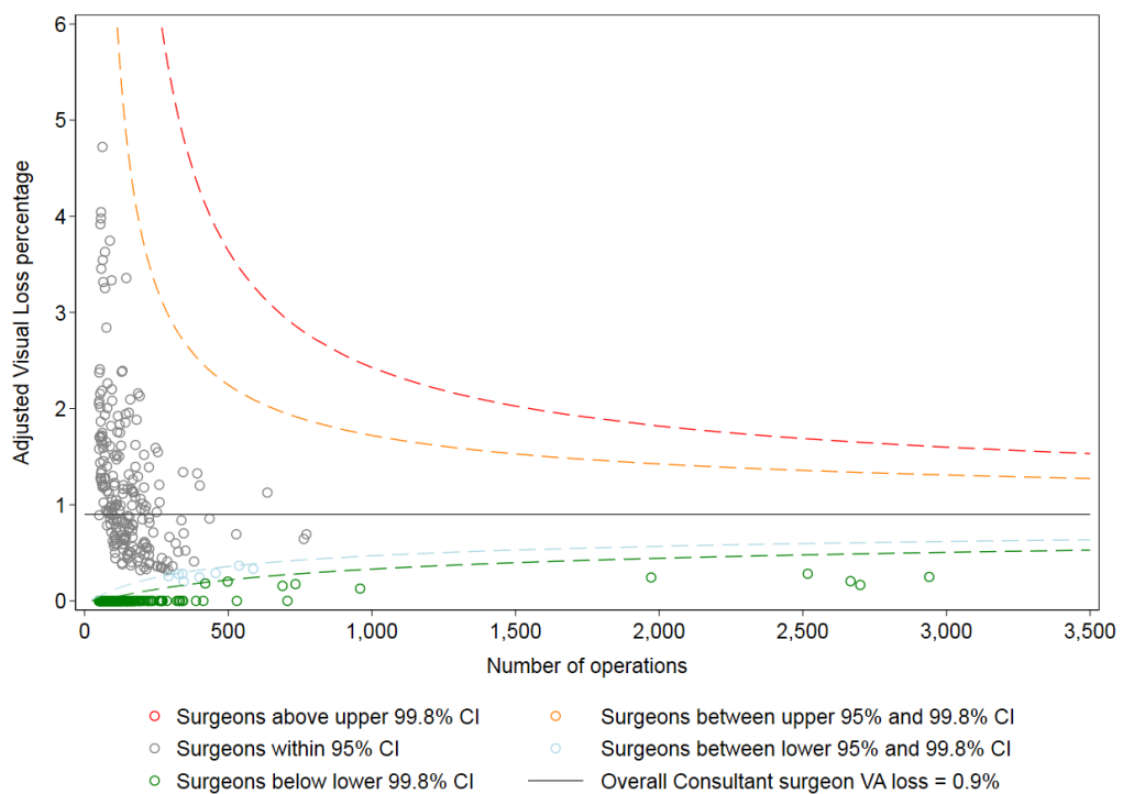
Figure 5: adjusted for case complexity VA loss graph for consultant and career grade non-consultant surgeons; data for audit year 3.
